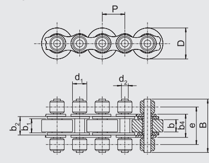
Design OS devoid of washers
