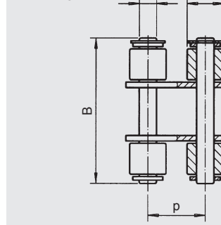
Connecting link
